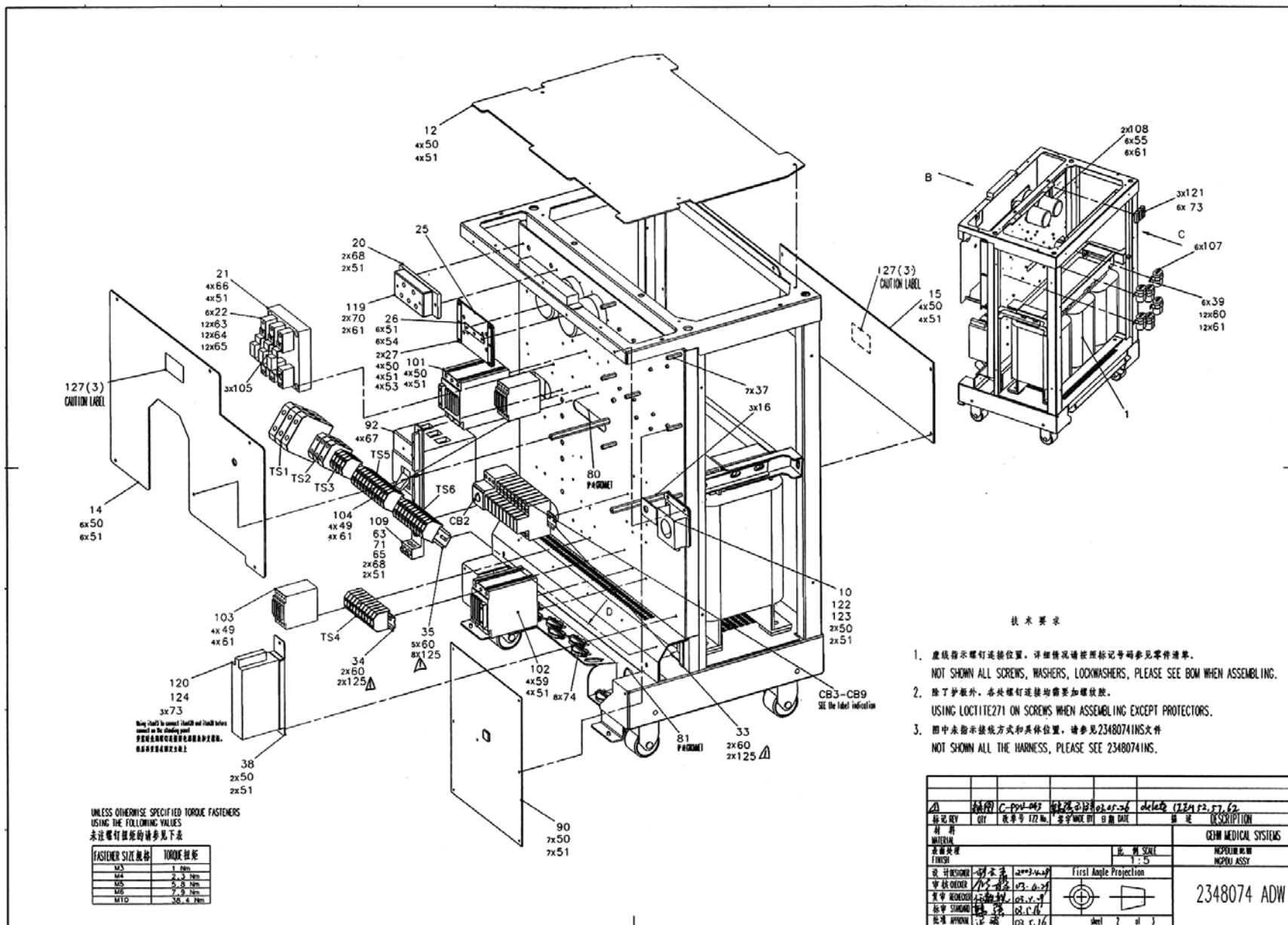
Figure 3-2 NGPDU Assembly 1 (2348074, sheet 2, rev 1)
